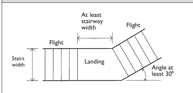
Diagram 3 Change of direction Par. 1.1.12 in places of assembly
